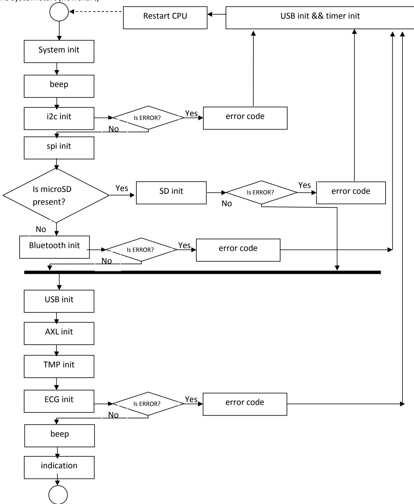
Firmware system start (flowchart)
